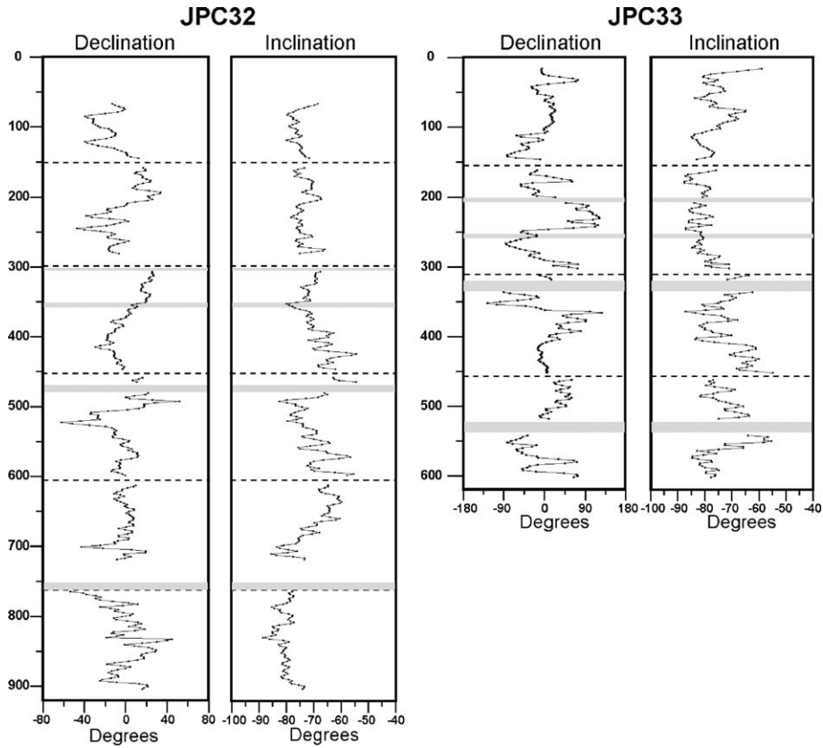
Figure 5. Declination and inclination determined from AF demagnetization at 20 mT. Declinations have been rotated to obtain a whole-core average value of 0°. Dashed horizontal lines indicate core section boundaries. Grey horizontal lines indicate position of ash layers.
