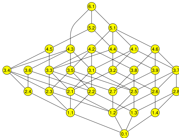
Figure 9: The Hasse diagram for \mathcal{P}_6
