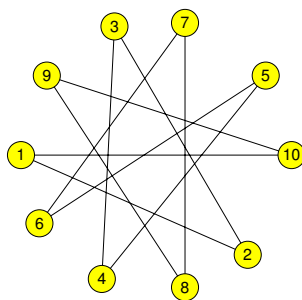
Figure 11: A realization of C_{10} with the maximum number of crossings
