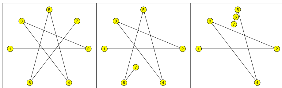
Figure 10: Geometric realizations of P_7 with 10 crossings, 6 crossings, and 3 crossings
