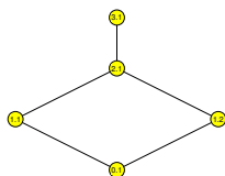
Figure 7: The Hasse diagram for \mathcal{P}_5
