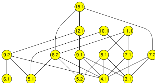
Figure 13: The Hasse diagram for \mathcal{K}_6
