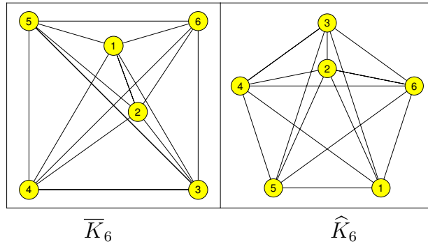
Figure 4: Vertex labels giving a geometric homomorphism from \overline{K}_6 to \widehat{K}_6
