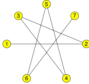
Figure 6: \overline{P}_7 with the maximum number of crossings
