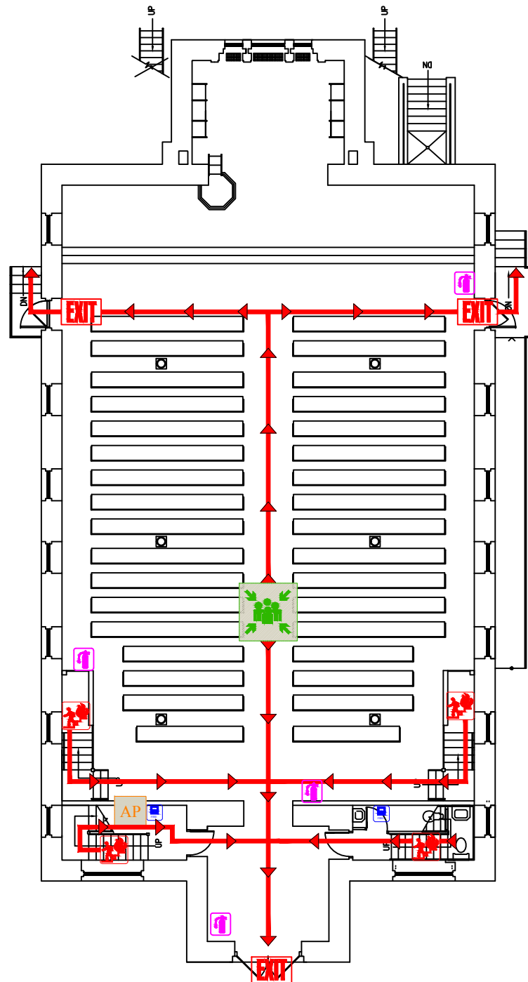
First Floor
