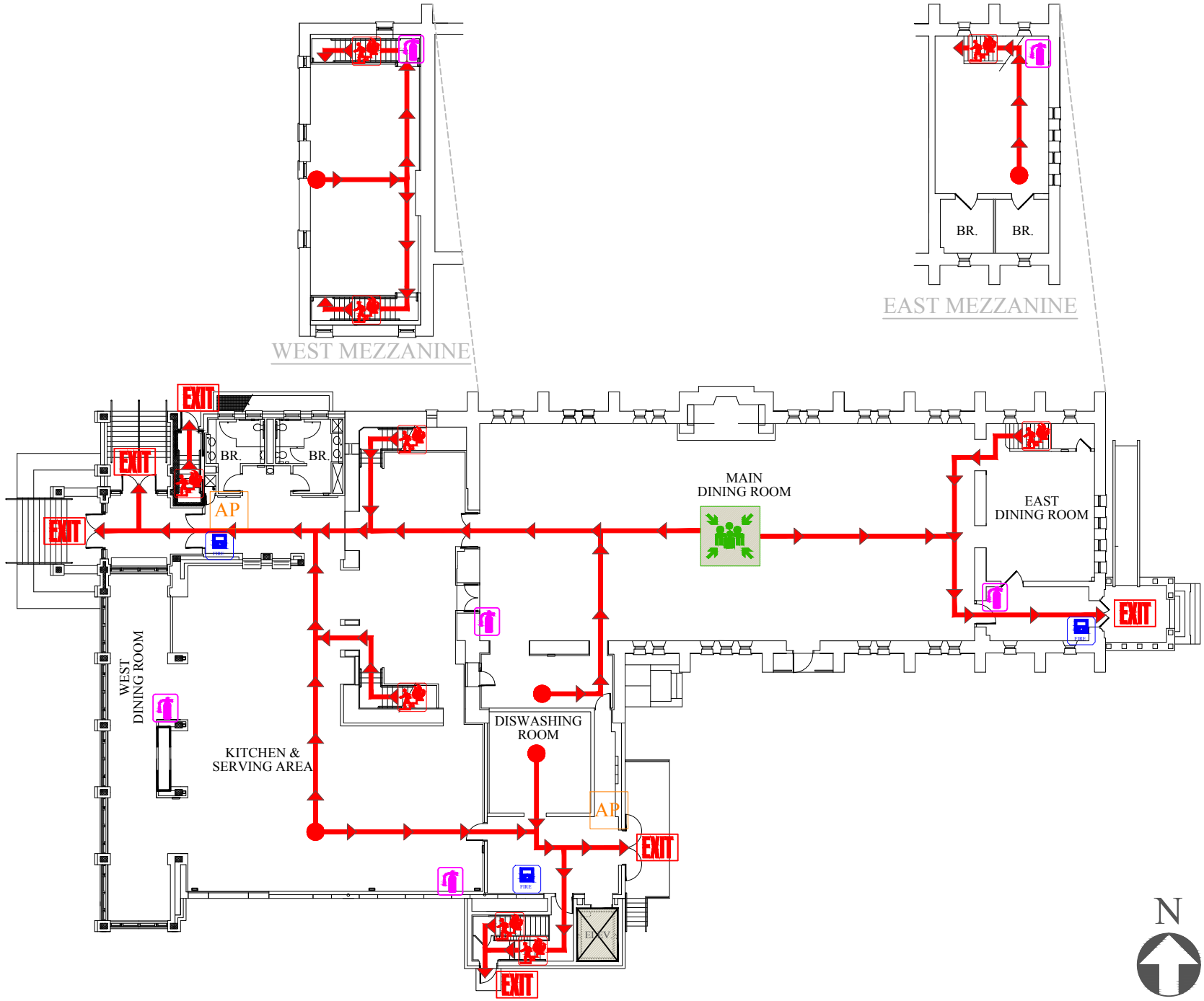
Level 1 and East / West Mezzanine
